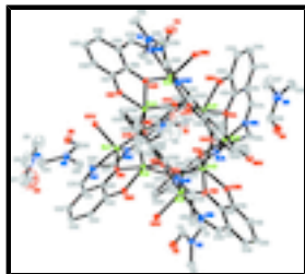
Fig. 1. Structure of the title compound, with thermal ellipsoids drawn at 30% probability level. Hydrogen atoms are omitted for clarity.
